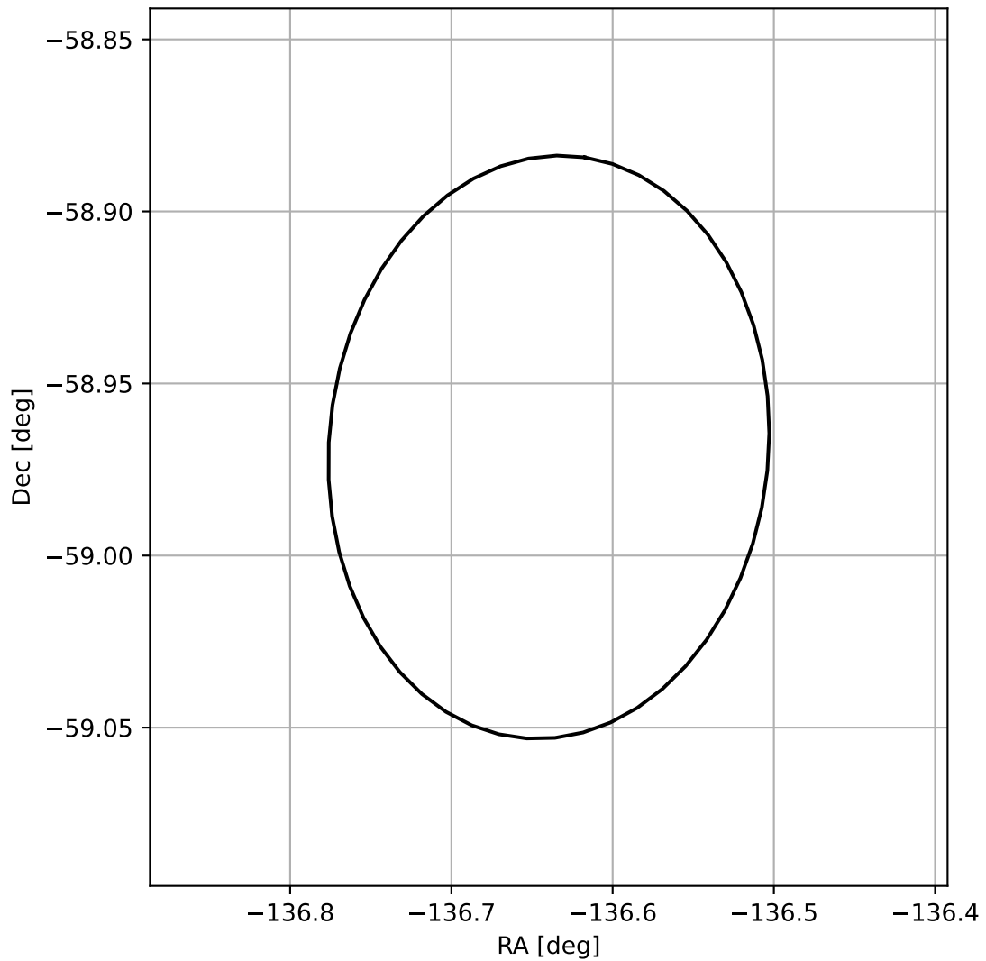
4FGL J1453.4-5858
