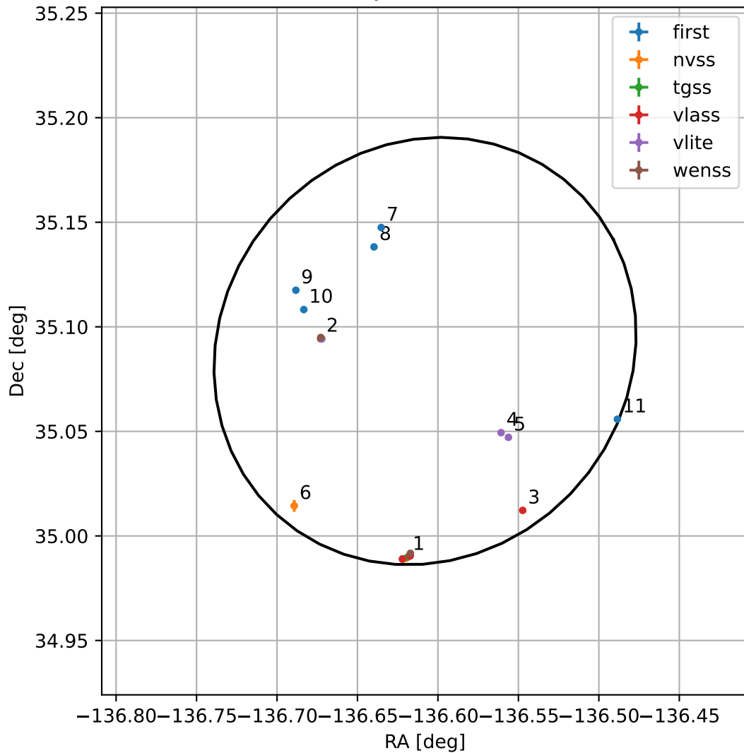
4FGL J1453.5+3505
