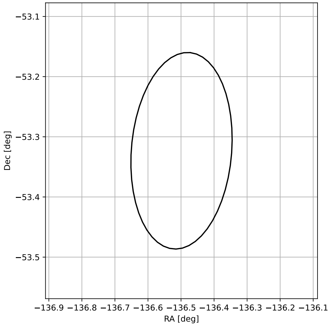
4FGL J1454.0-5319
