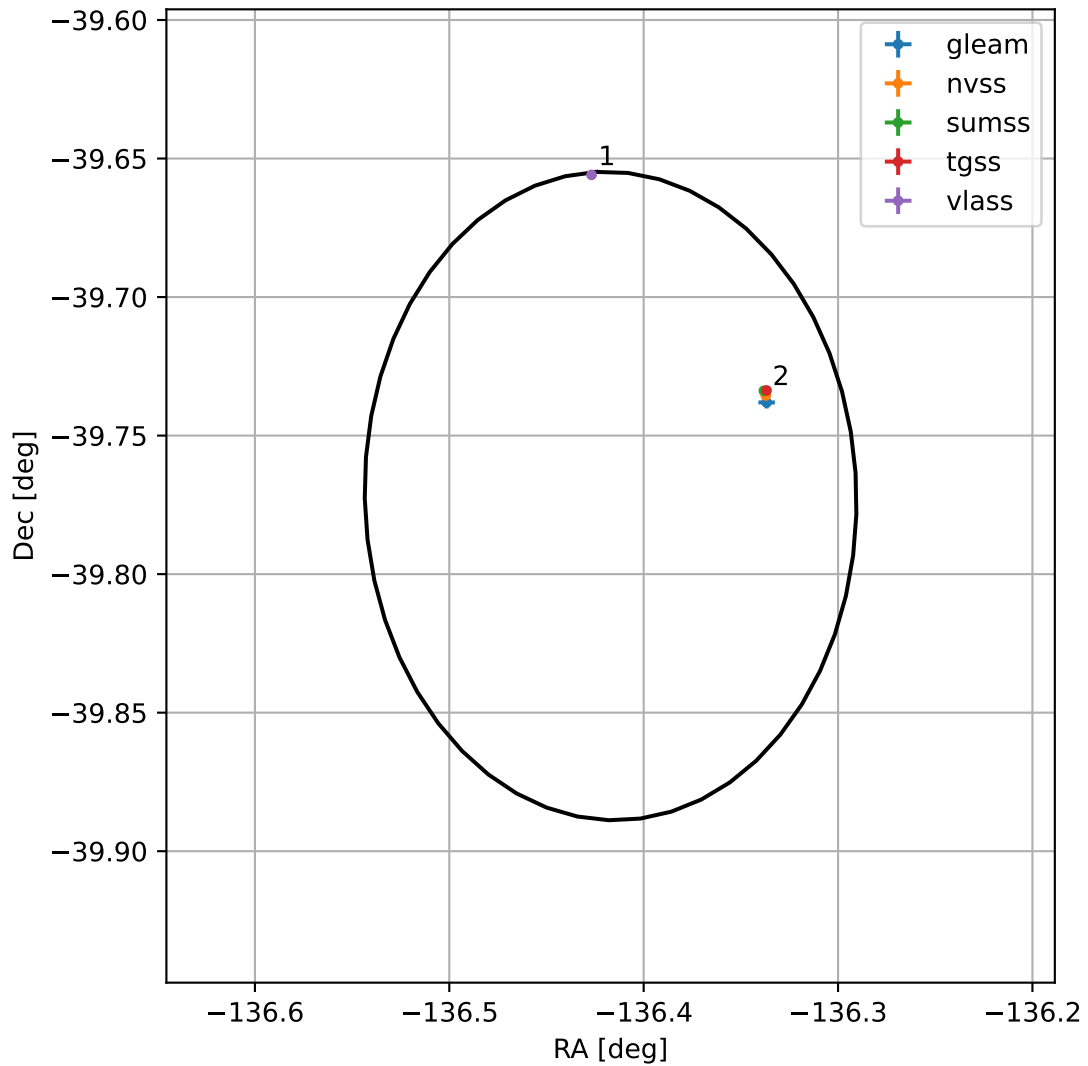
4FGL J1454.3-3946
