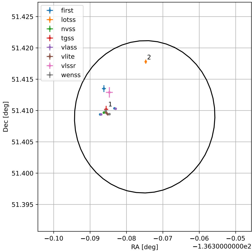
4FGL J1454.4+5124
