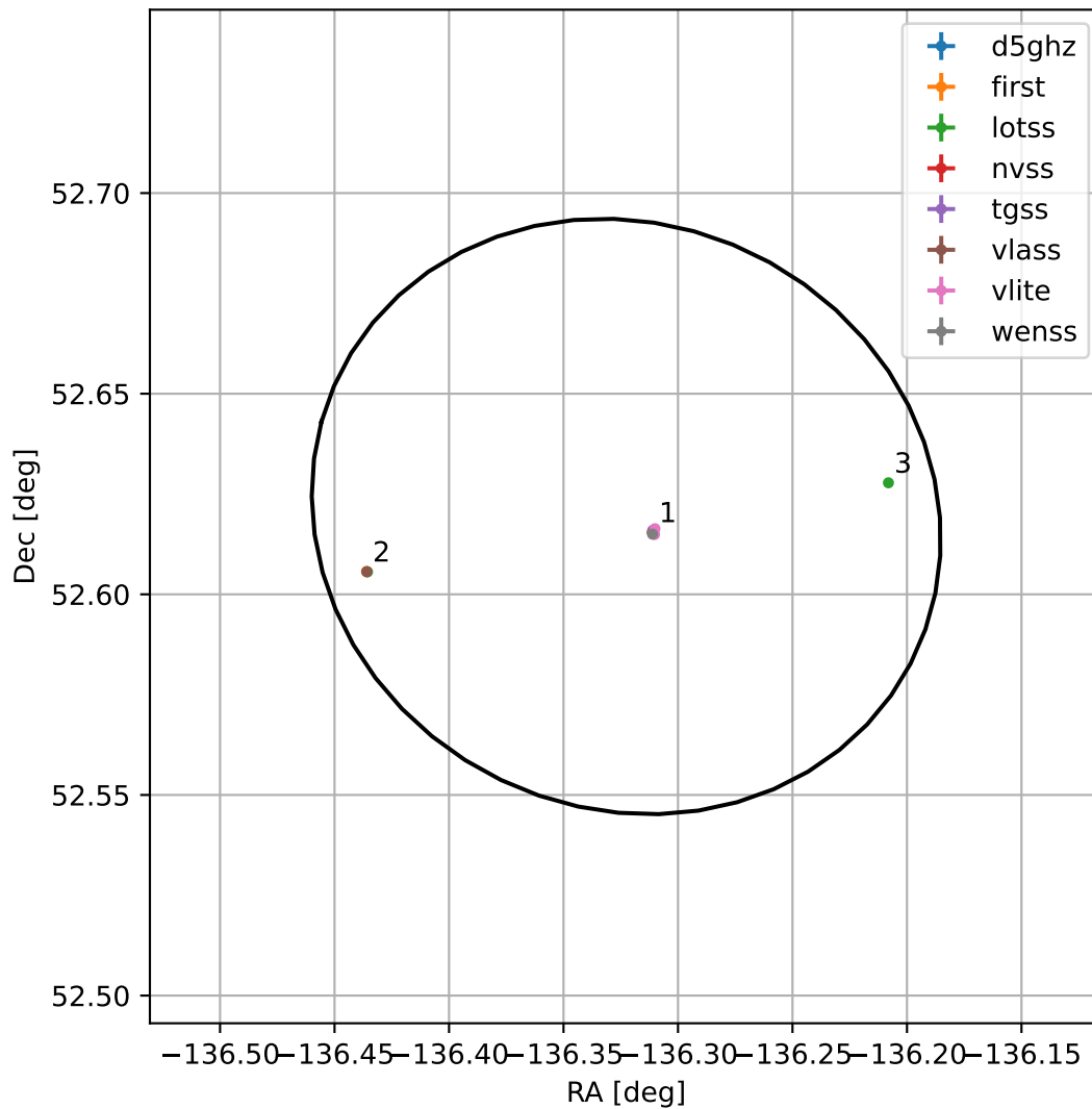
4FGL J1454.7+5237
