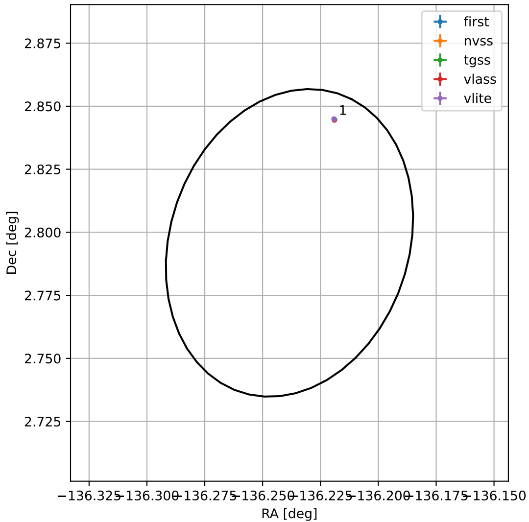
4FGL J1455.0+0247
