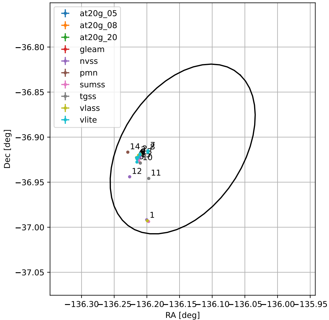
4FGL J1455.4-3654
