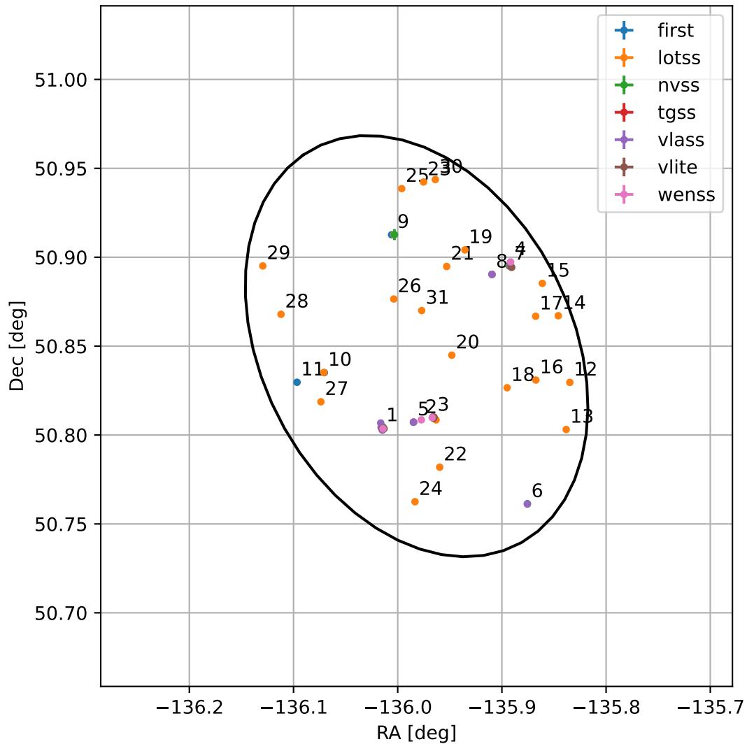
4FGL J1456.0+5051
