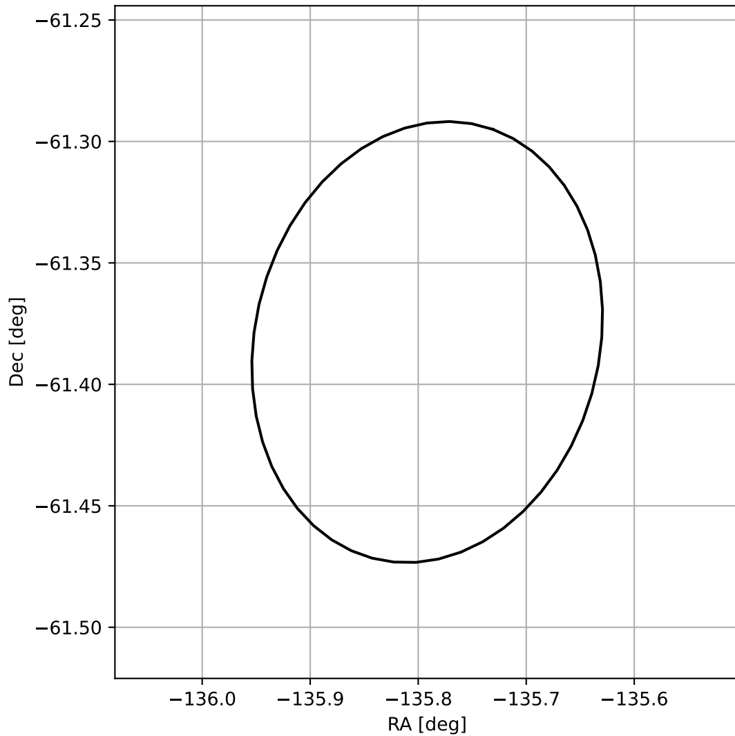
4FGL J1456.8-6122
