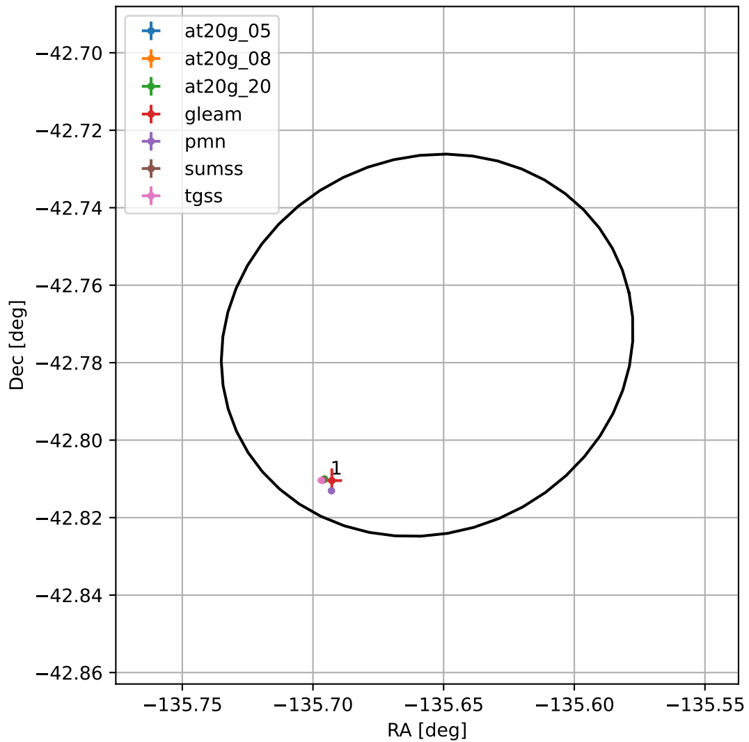
4FGL J1457.3-4246
