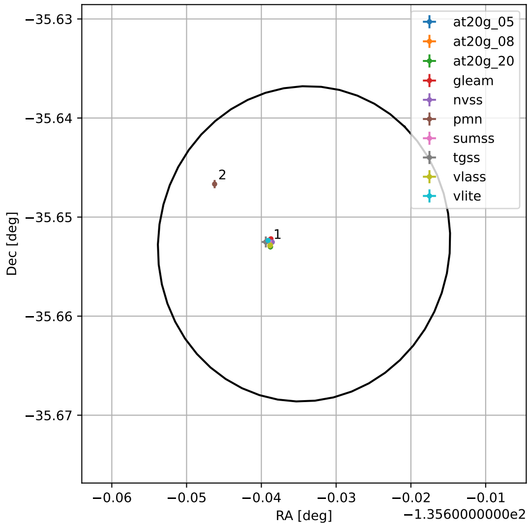
4FGL J1457.4-3539
