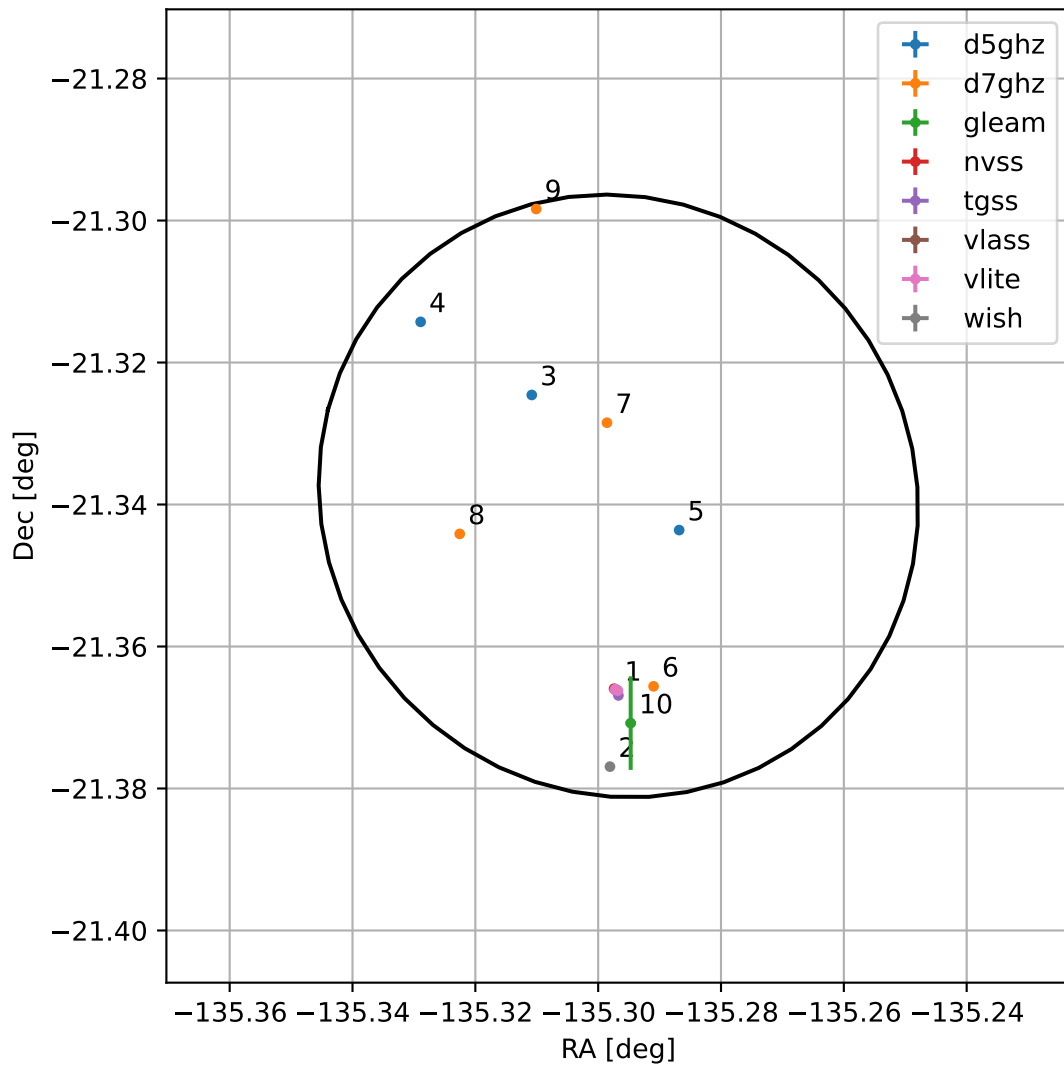
4FGL J1458.8-2120
