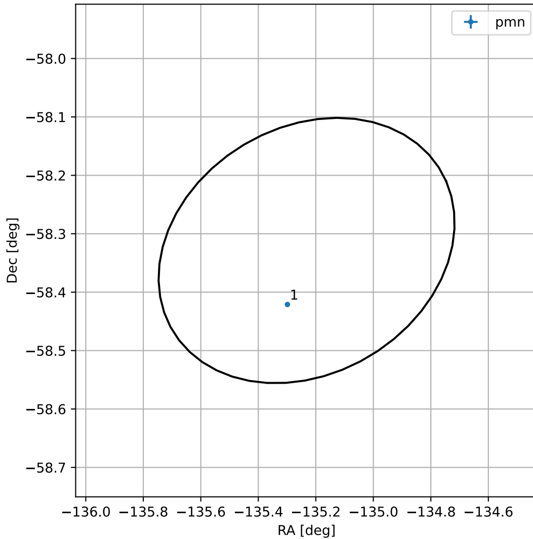
4FGL J1459.0-5819
