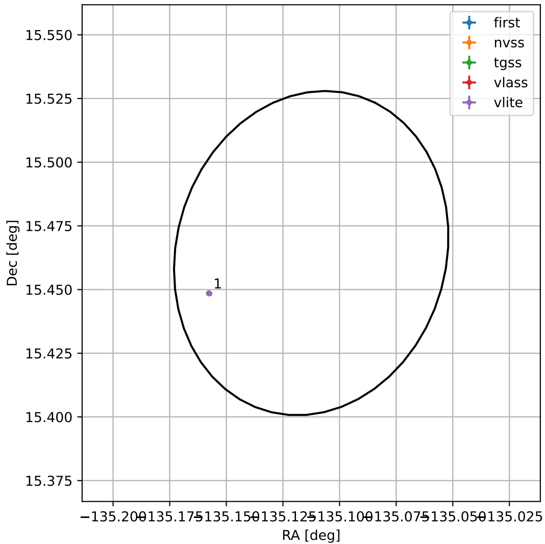
4FGL J1459.5+1527
