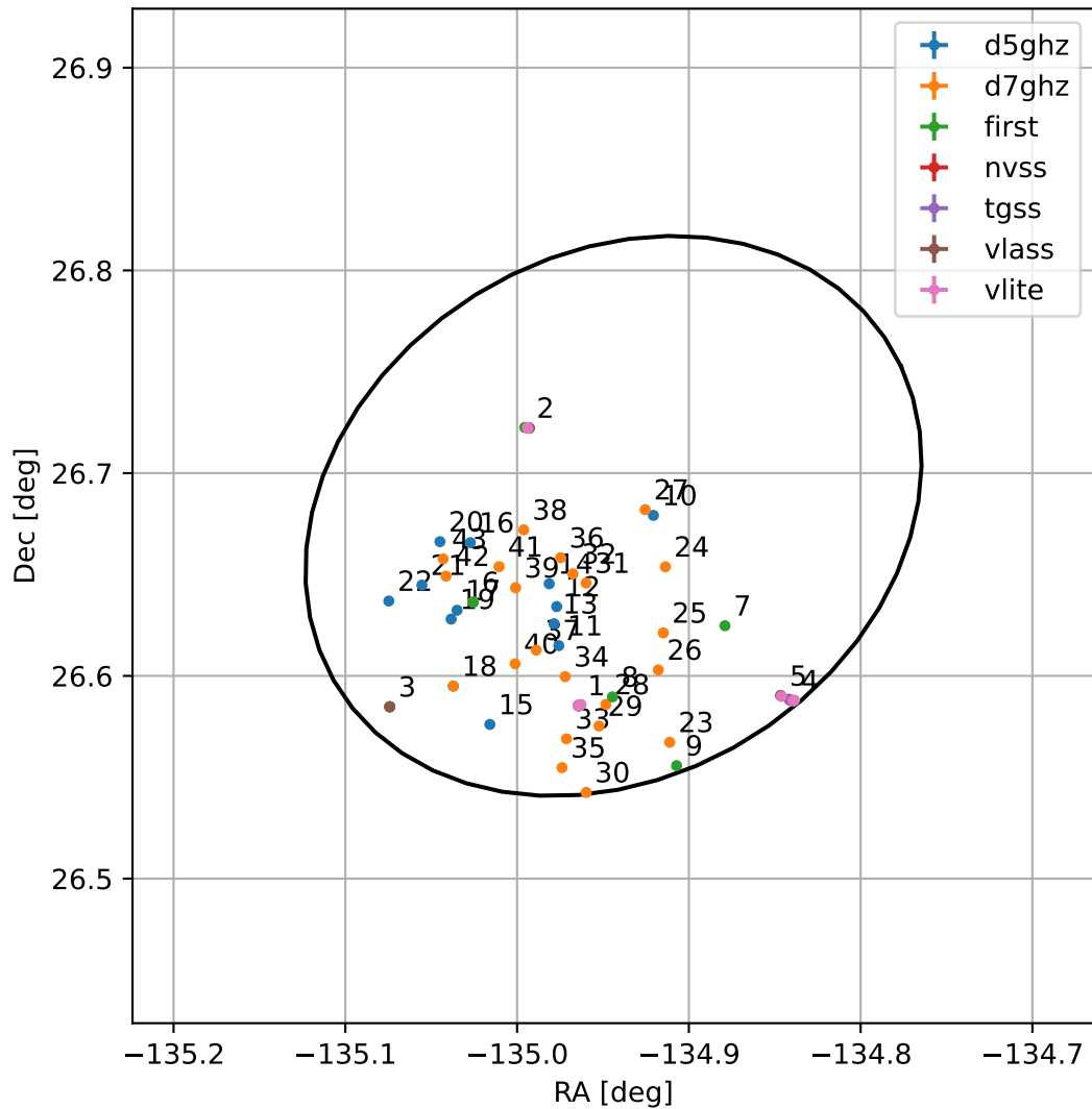
4FGL J1500.2+2640
