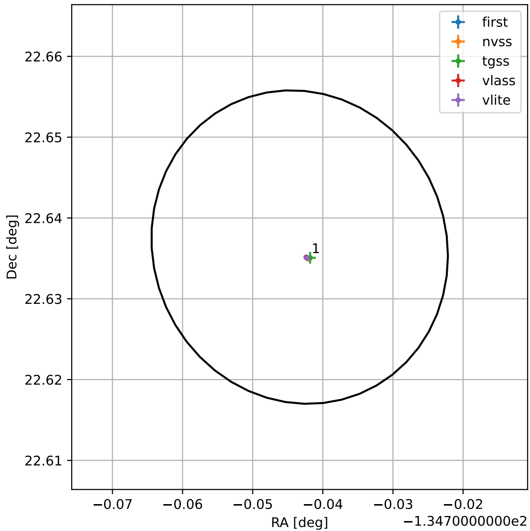
4FGL J1501.0+2238
