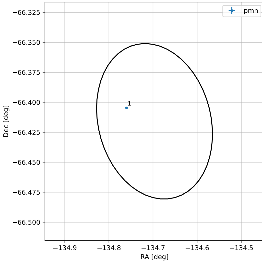
4FGL J1501.2-6624
