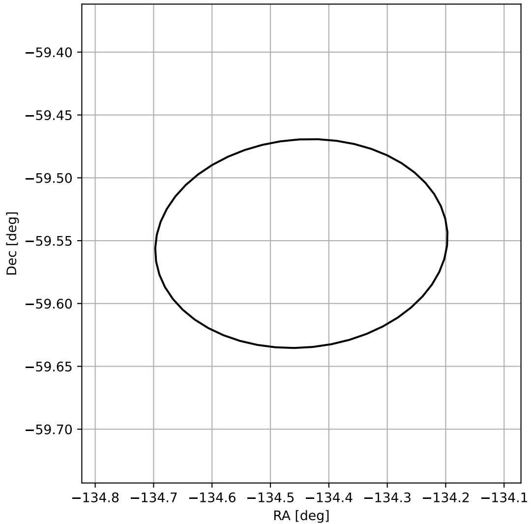
4FGL J1502.2-5933
