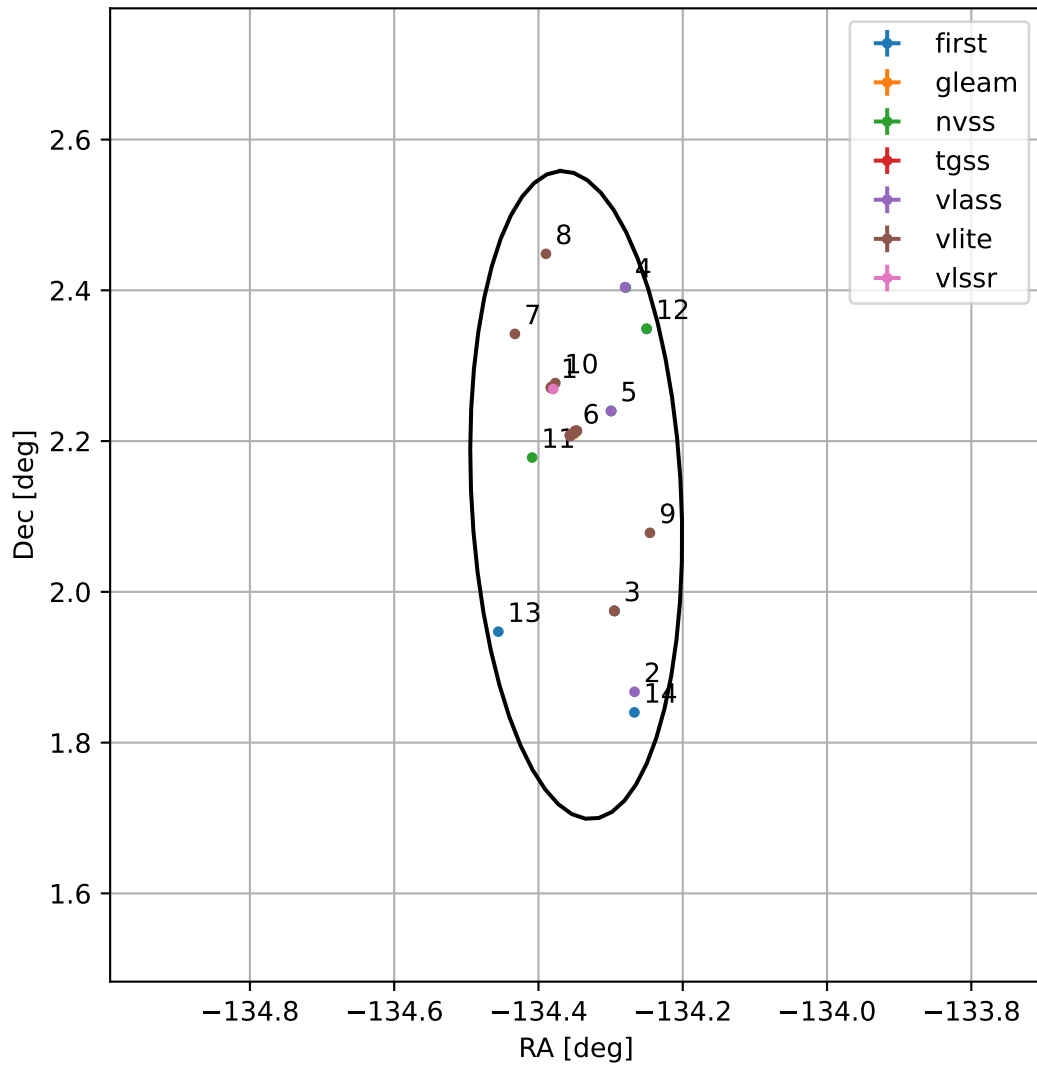
4FGL J1502.6+0207
