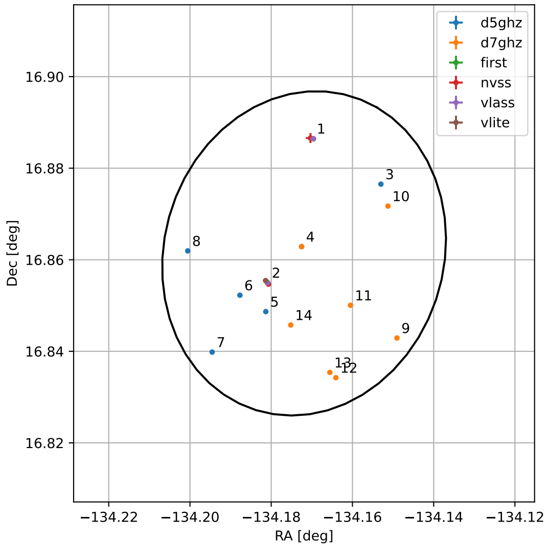
4FGL J1503.3+1651
