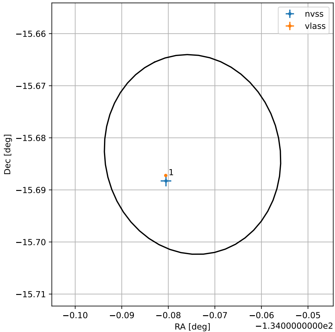
4FGL J1503.7-1540
