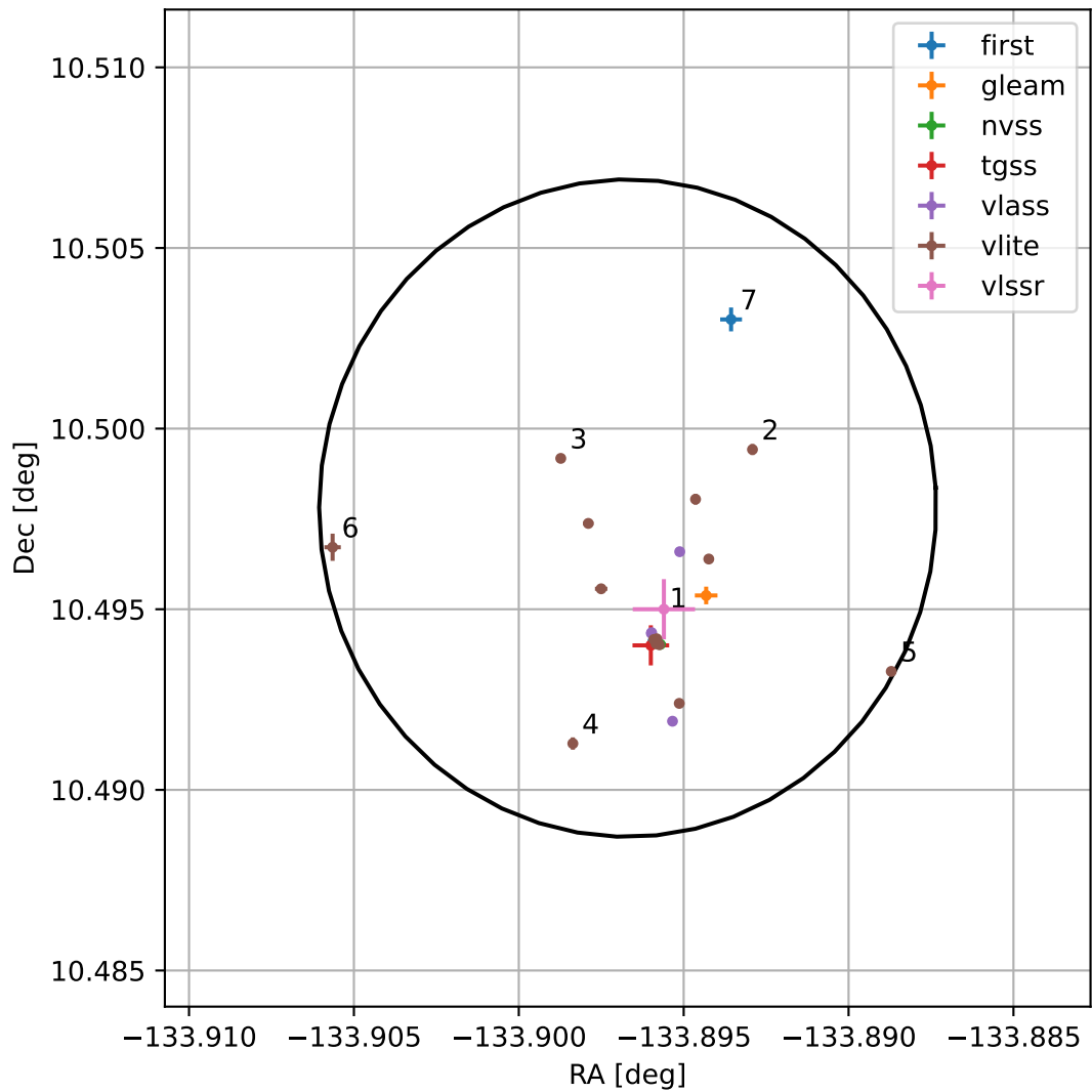
4FGL J1504.4+1029
