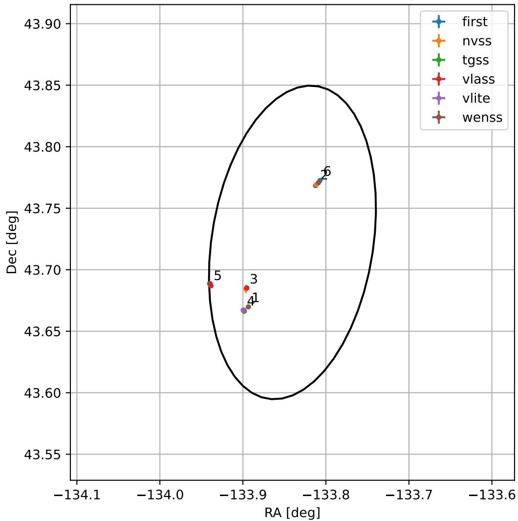
4FGL J1504.6+4343
