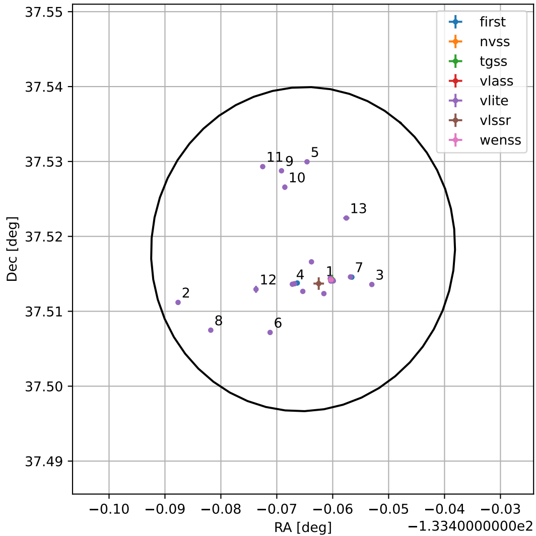
4FGL J1506.1+3731
