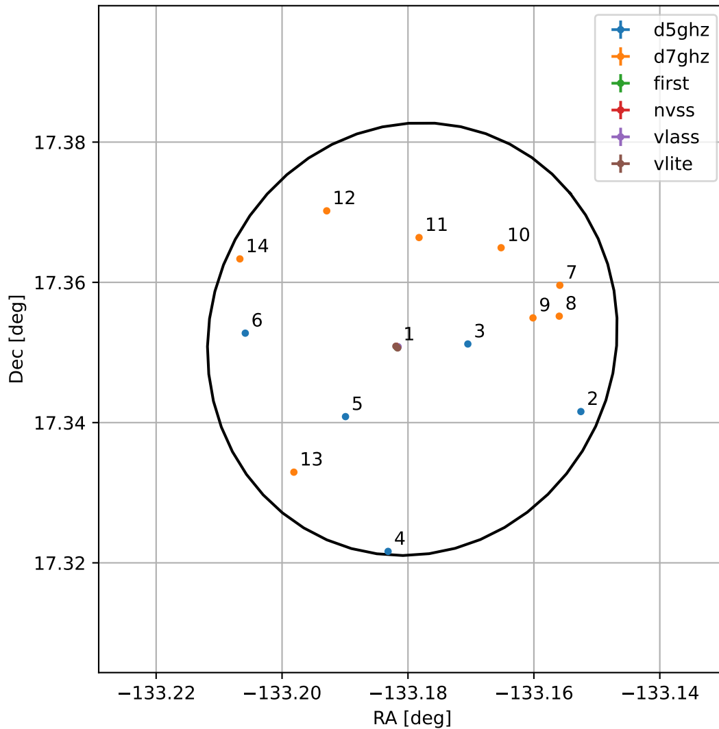
4FGL J1507.2+1721
