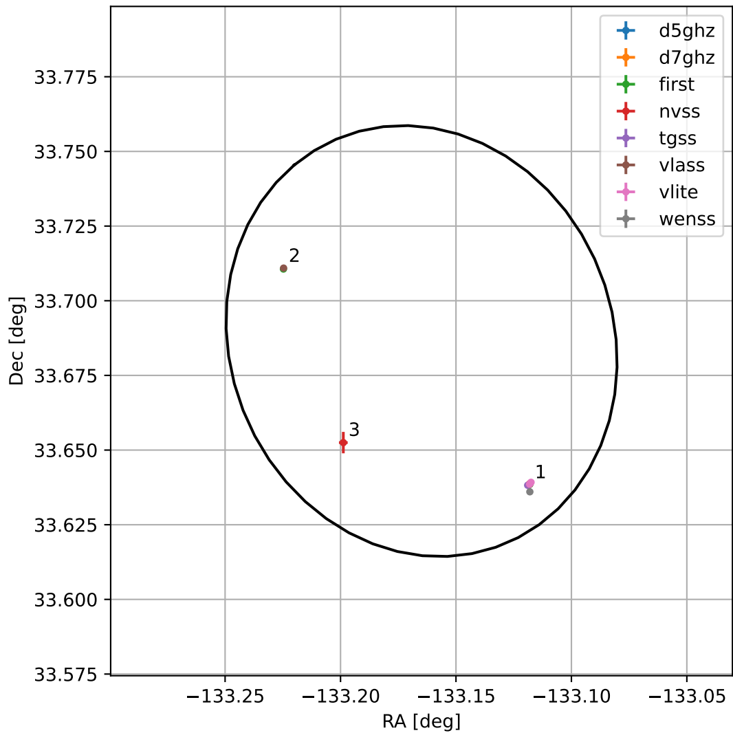
4FGL J1507.3+3341
