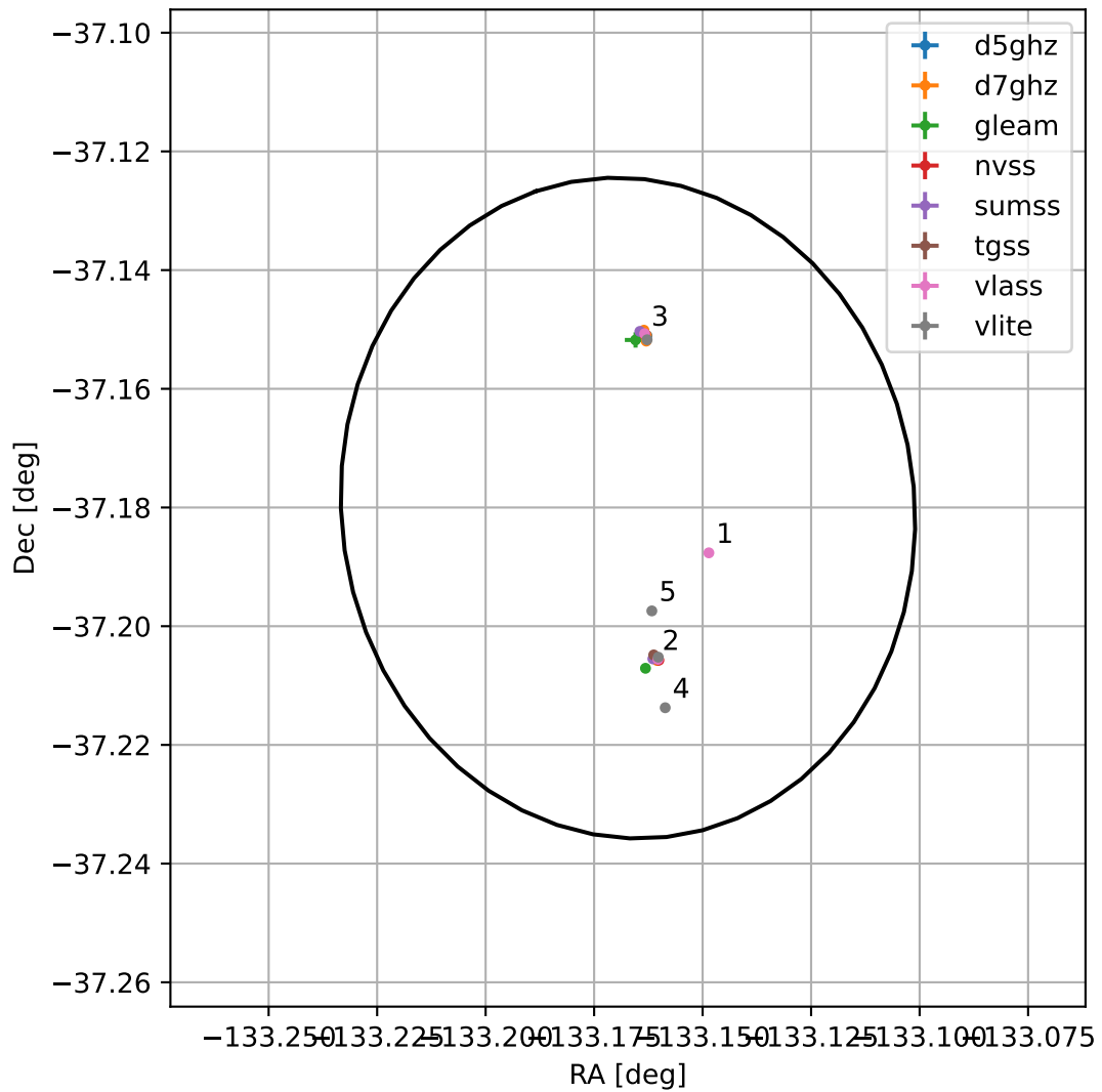
4FGL J1507.3-3710
