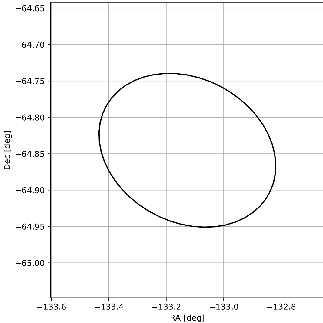
4FGL J1507.4-6450
