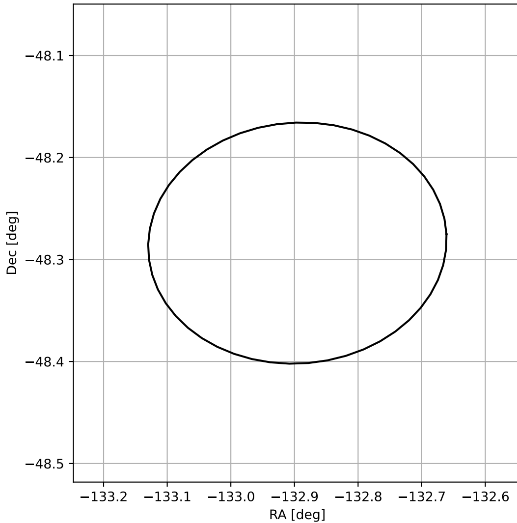
4FGL J1508.4-4817
