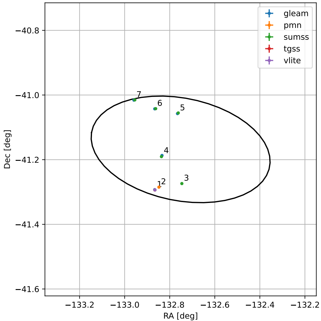
4FGL J1508.9-4110
