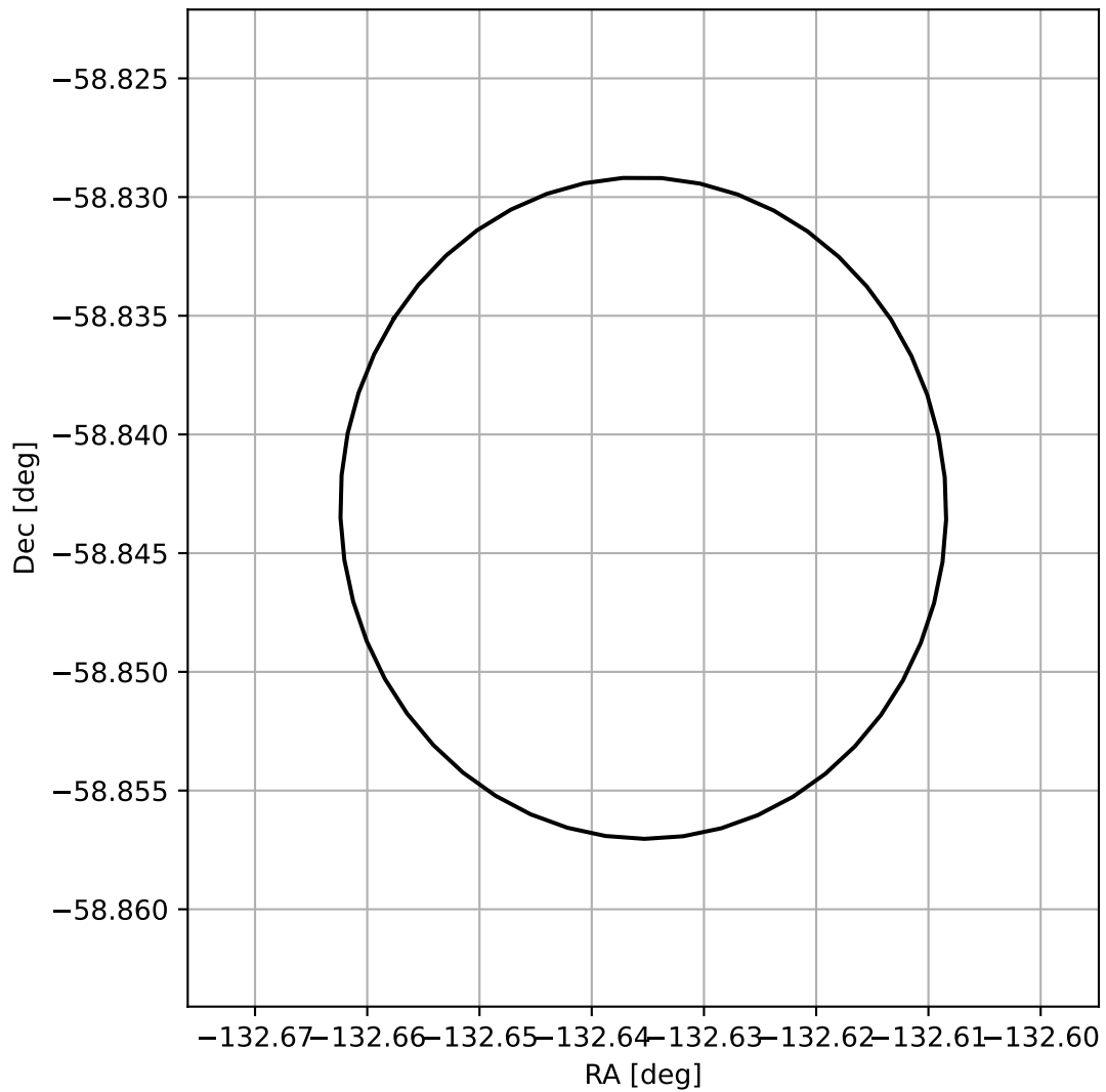
4FGL J1509.4-5850
