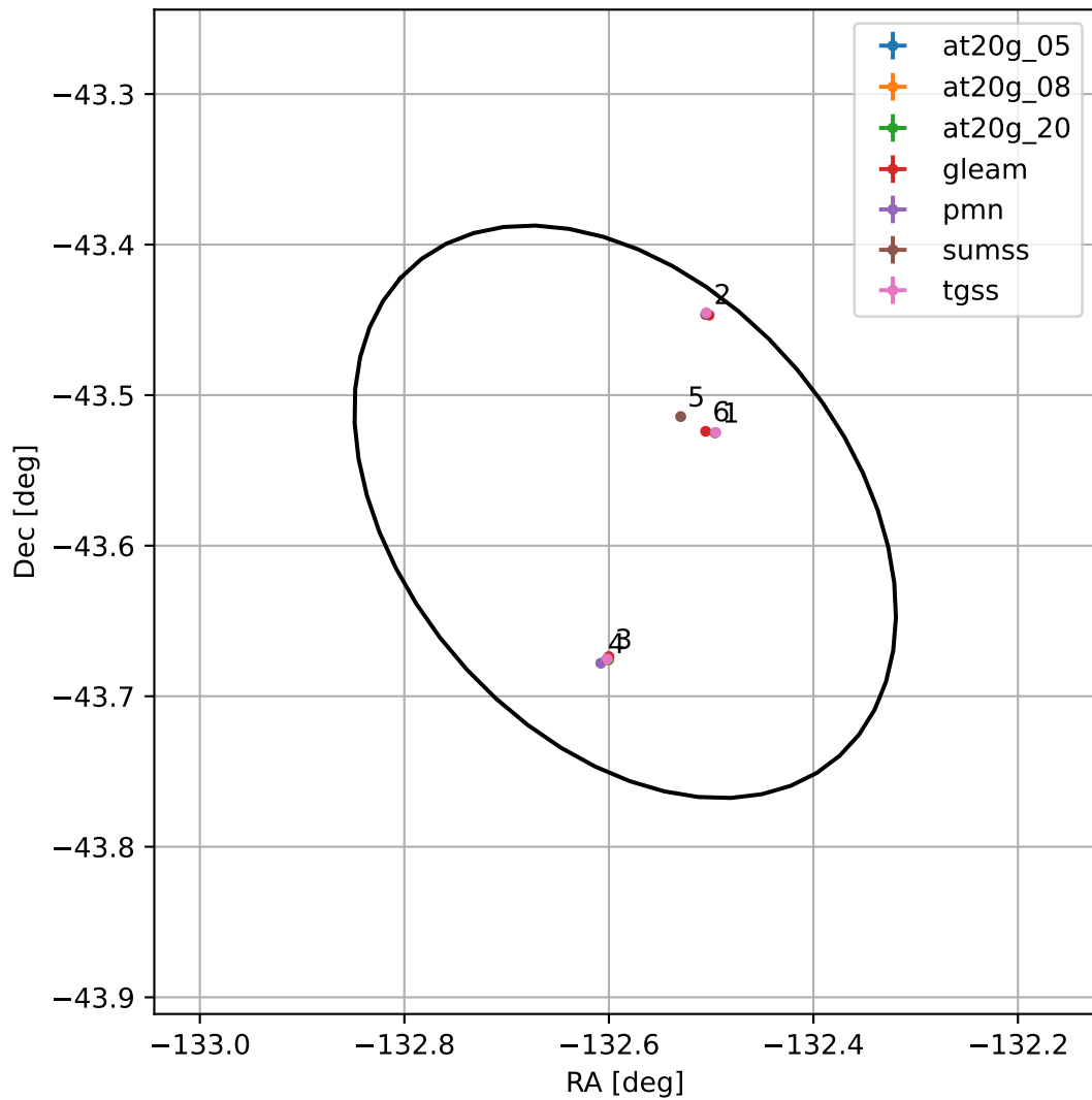
4FGL J1509.6-4334
