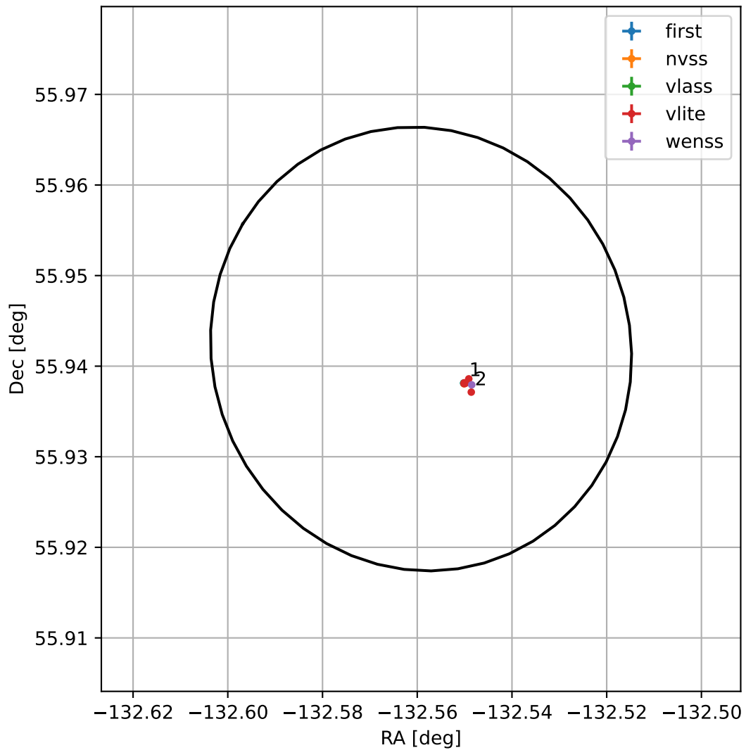
4FGL J1509.7+5556
