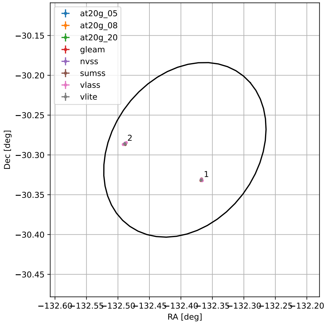
4FGL J1510.4-3017
