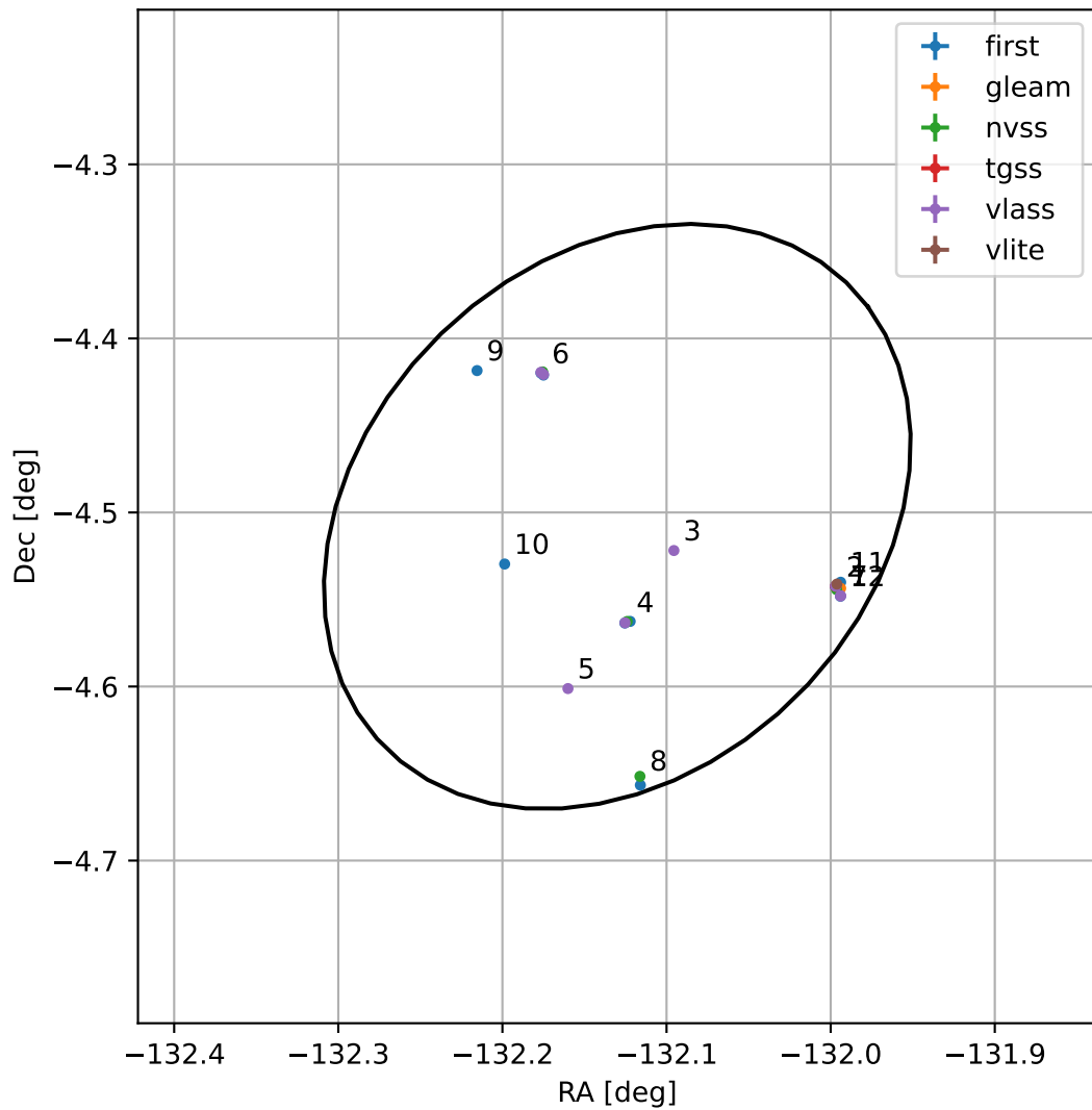
4FGL J1511.4-0430
