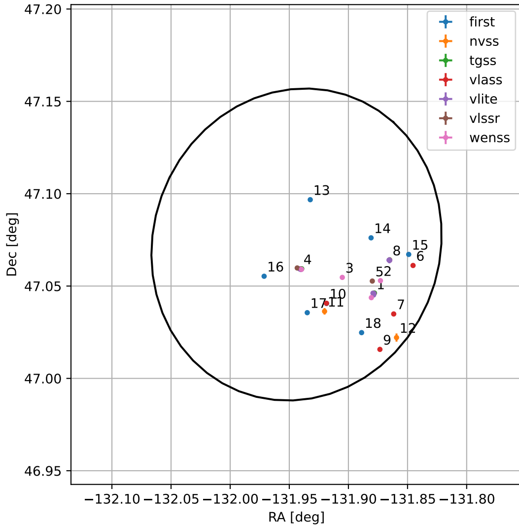
4FGL J1512.2+4704
