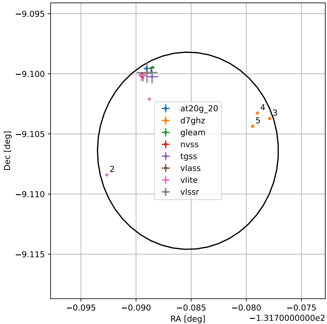
4FGL J1512.8-0906
