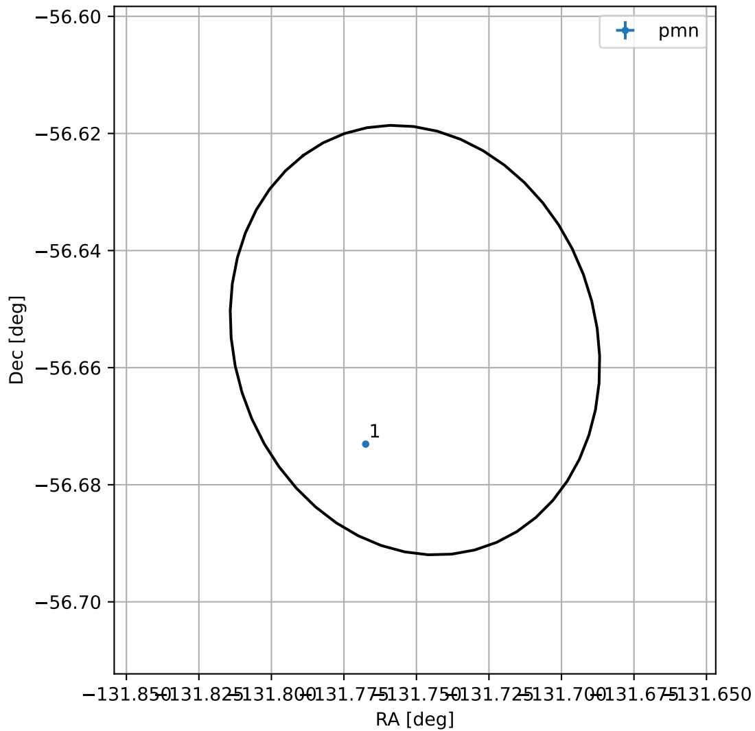
4FGL J1512.9-5639
