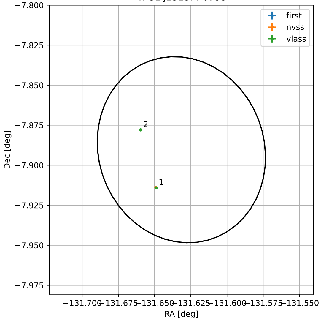
4FGL J1513.4-0753
