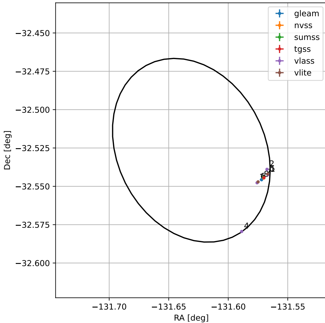
4FGL J1513.4-3231
