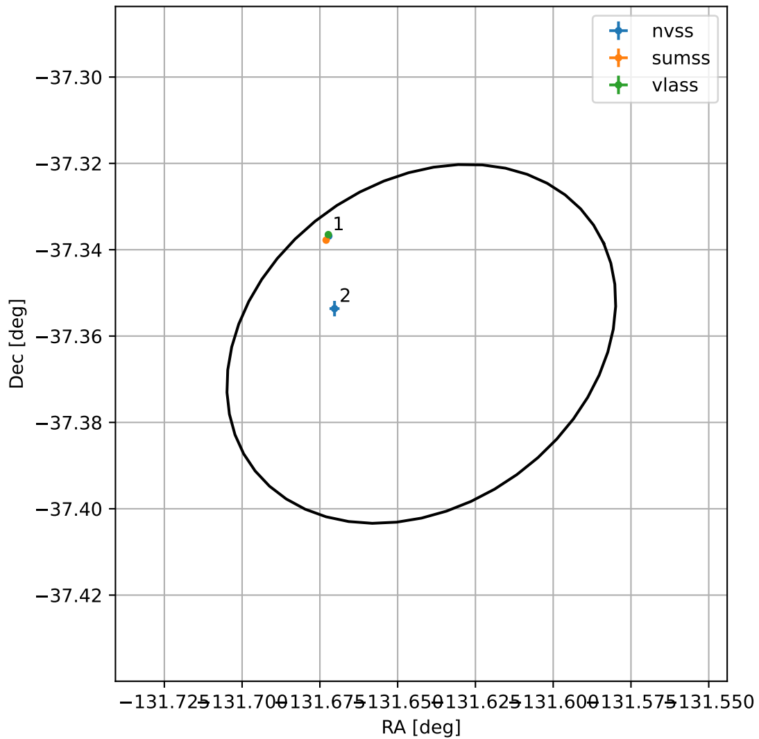
4FGL J1513.4-3721
