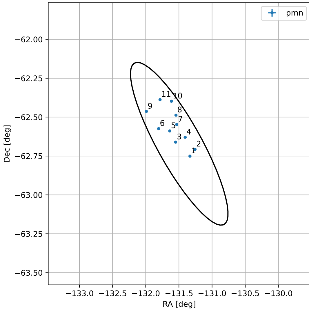
4FGL J1514.0-6240
