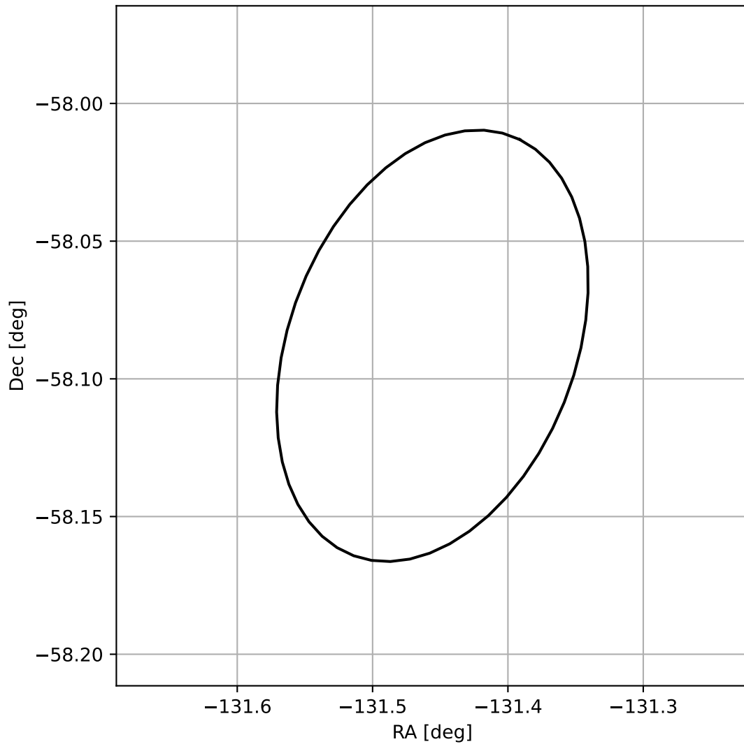
4FGL J1514.1-5805
