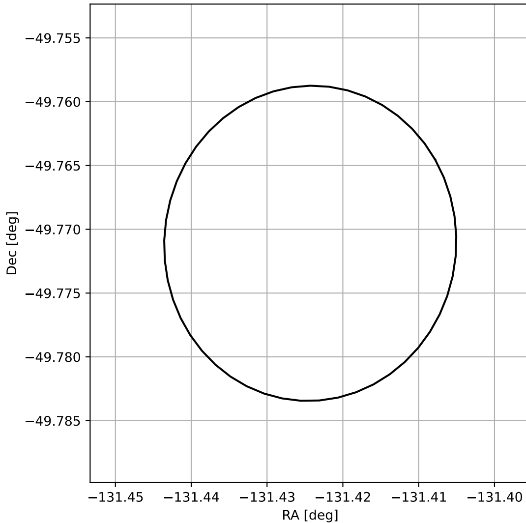
4FGL J1514.3-4946
