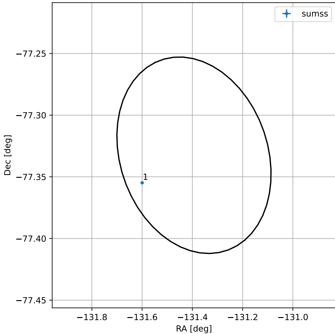
4FGL J1514.4-7719
