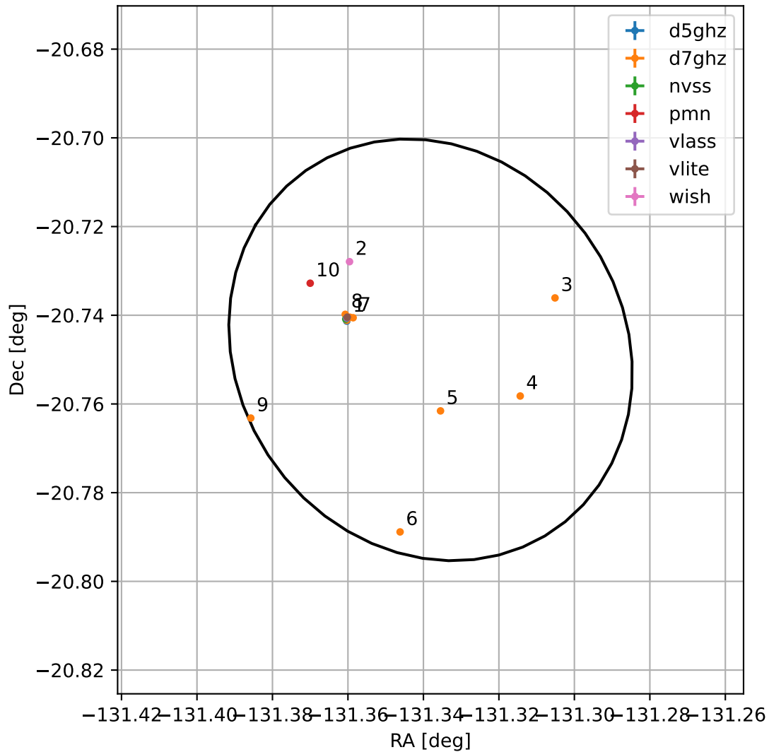
4FGL J1514.6-2044
