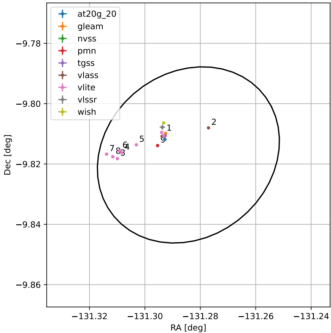
4FGL J1514.8-0949
