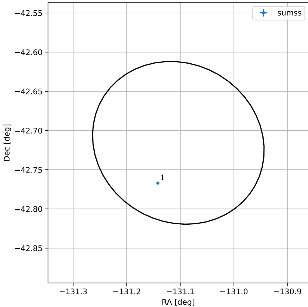
4FGL J1515.5-4242
