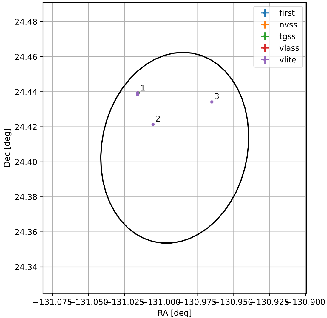
4FGL J1516.0+2424
